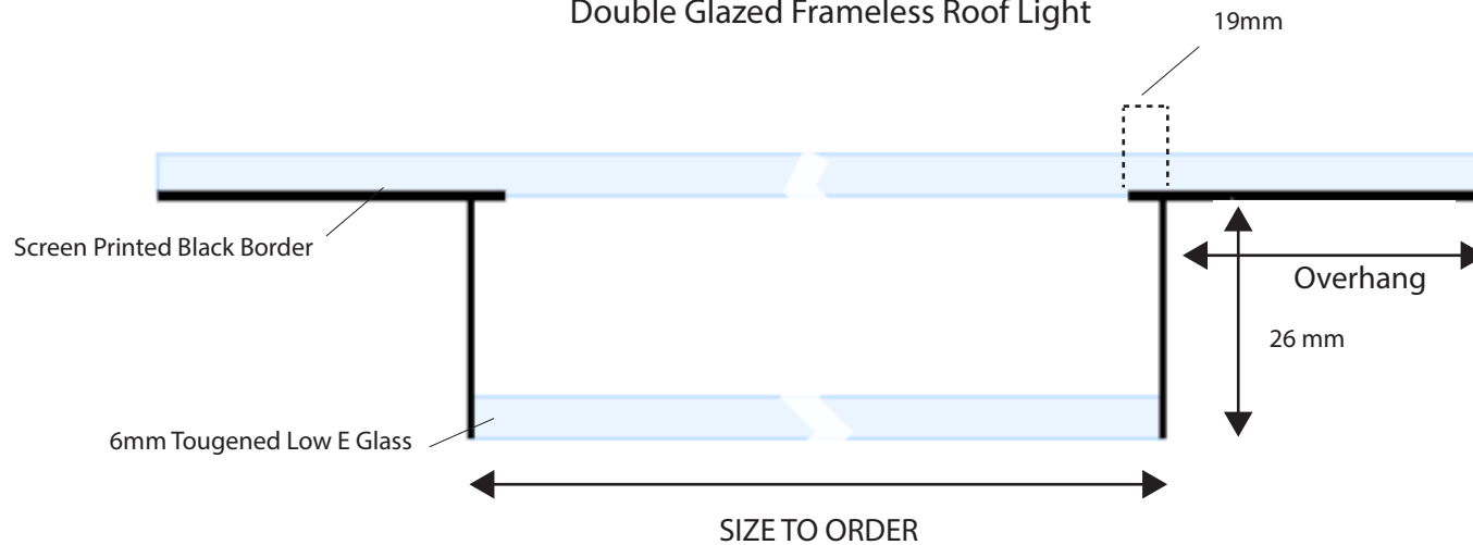
Double Glazed Frameless Roof Light
